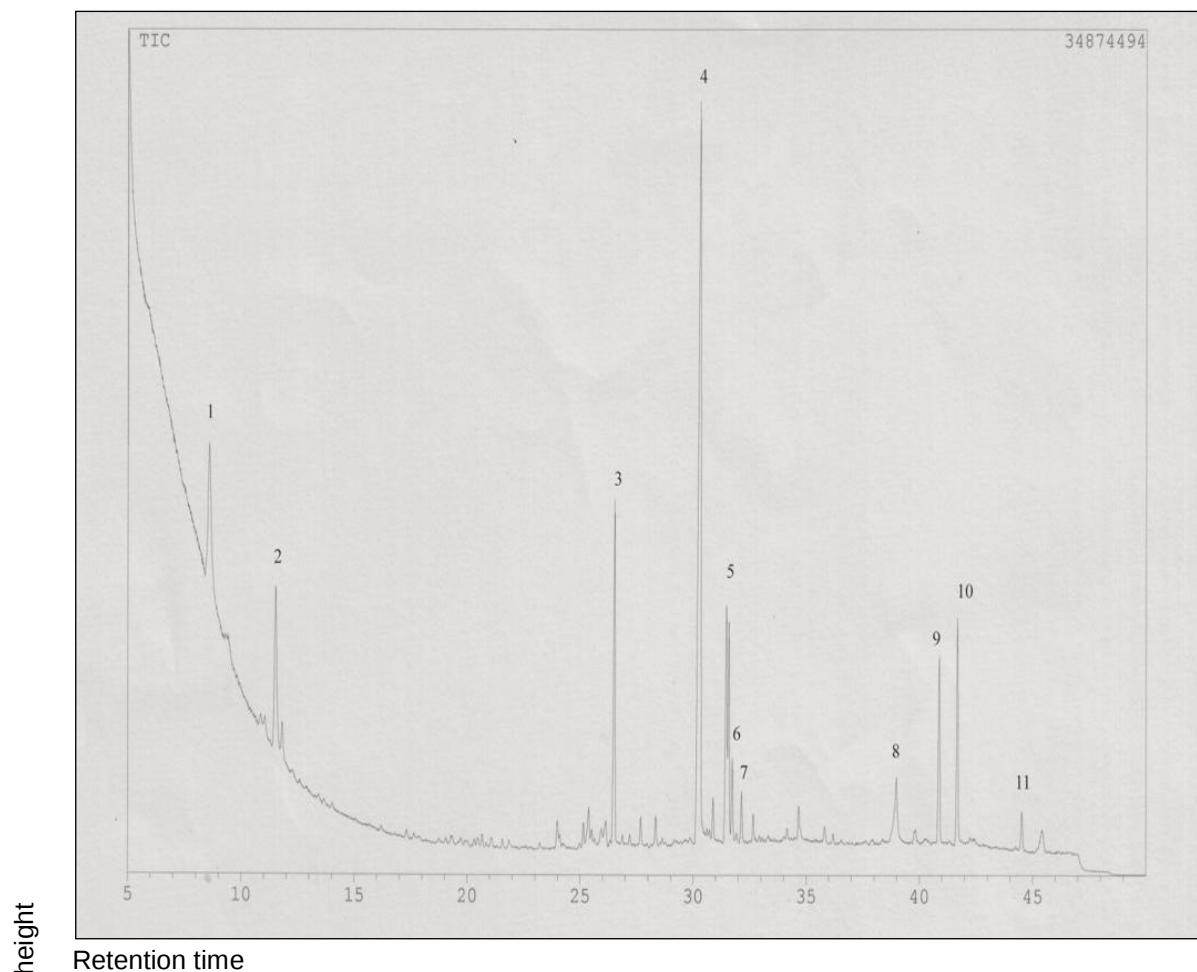
Figure 4. Chromatogram of carrot in GCMS
