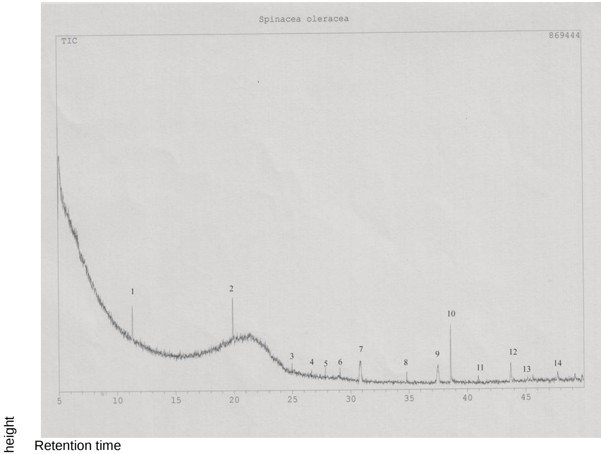
Figure 2. Chromatogram of spinach in GCMS
