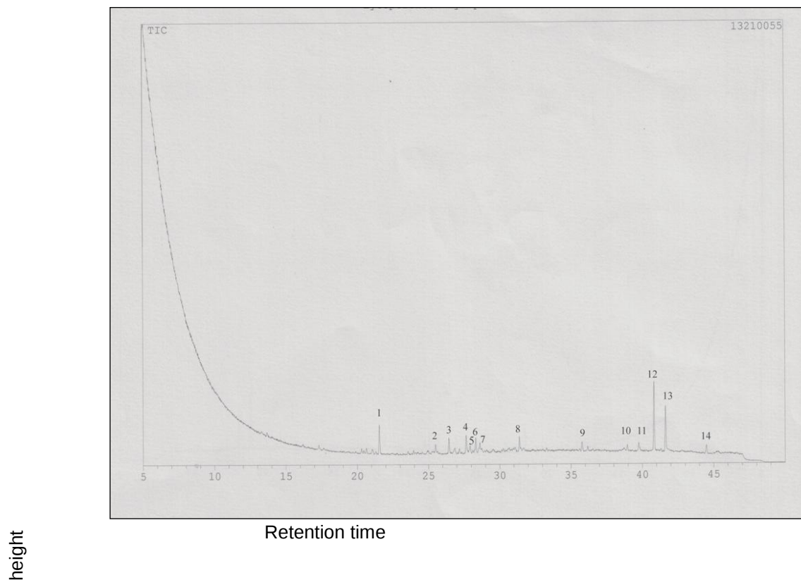
Figure 1. Chromatogram of tomato in GCMS
