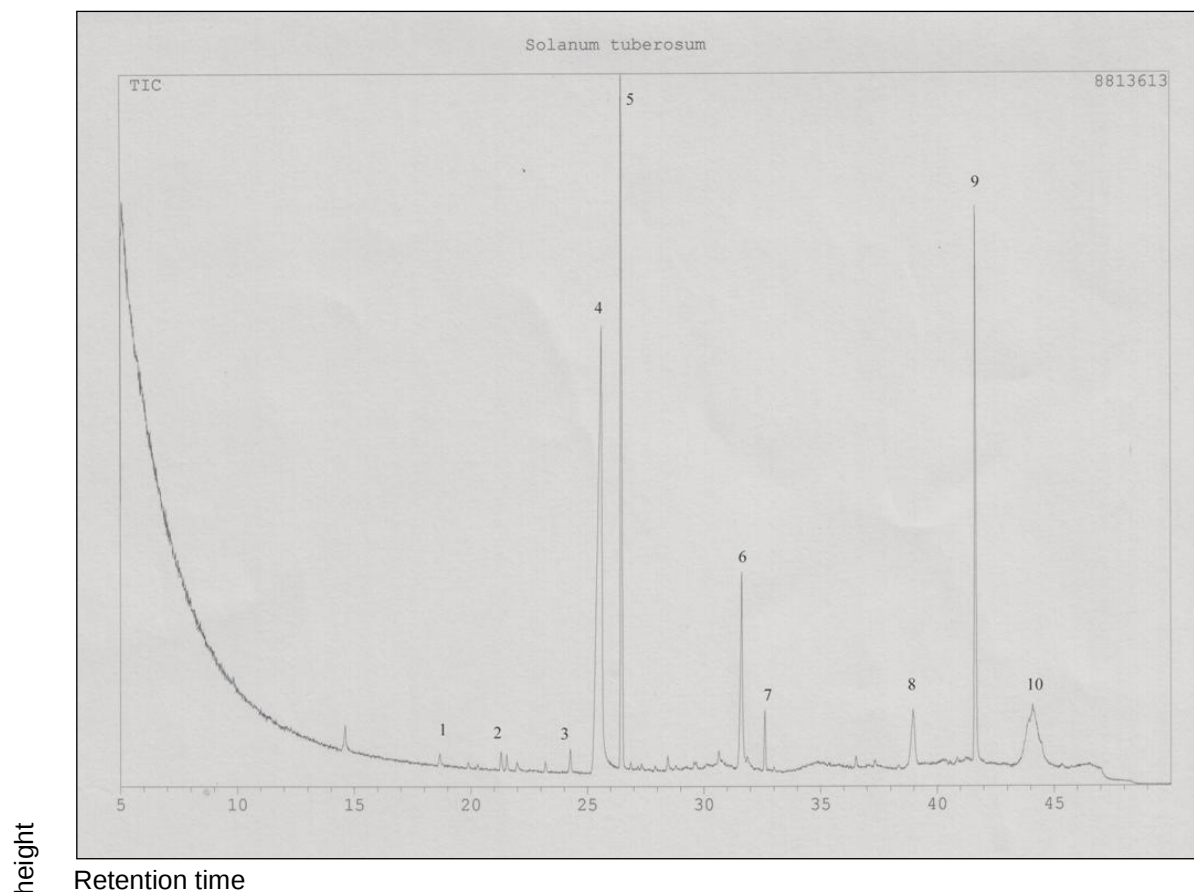
Figure 3. Chromatogram of Potato in GCMS
