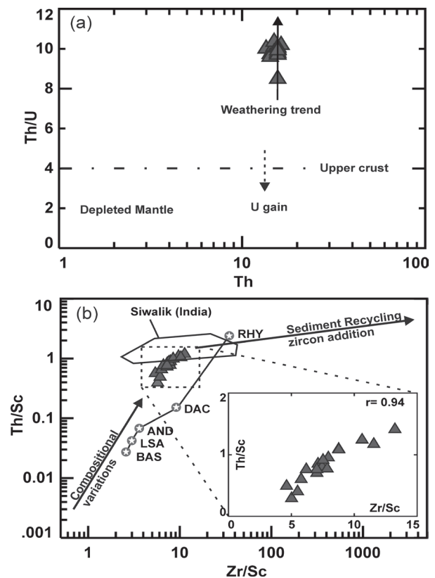
Fig. 7: (a) Th/U vs. Th plot for the Tista river sediments following fields and trends from Gu et al. (2002) (b) Th/Sc-Zr/Sc diagram (McLennan et al. , 1993) for the river sediments. Stars: BAS (basalt), LSA (low silica andesite), DAC (dacite) and RHY (rhyolite) as plotted by Roser and Korsch (1999) and Siwalik Group (Ranjan and Banerjee, 2009).
