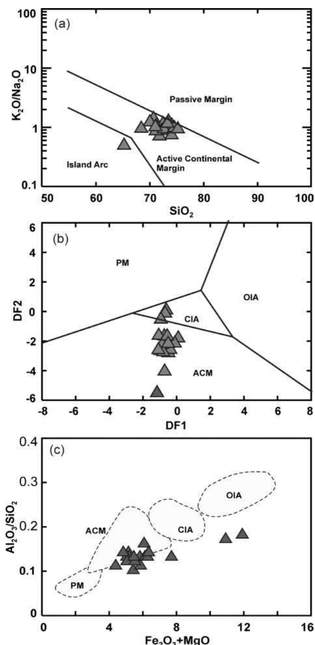
Fig. 11: (a) Tectonic setting discrimination diagram of \text{SiO}_2 vs. \log(\text{K}_2\text{O}/\text{Na}_2\text{O}) for the investigated river sediments (after Roser and Korsch, 1986) (b) and (c) after Bhatia, 1983, where PM= passive margin, ACM= active continental margin, IA= island arc, CIA= continental island arc, OIA= oceanic island arc.
