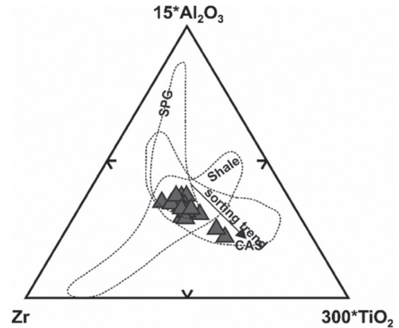
Fig. 6: Ternary plot of 15*Al_2O_3 -Zr- 300*TiO_2 for the studied sediments. Field of calc-alkaline granites marked as CAS, while field of strongly peraluminous granites denoted as SPG (after Garcia et al. , 1994).
