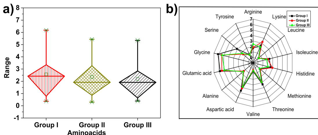
Fig. 2. a) Average amino acid in Group I, Group II, and Group-III of Hilsa fish, and b) Radar graph showing amino acid profile in different size groups of Hilsa fish.
