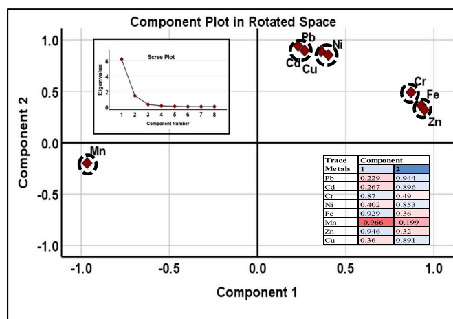
Fig. 4. Principal Component Plot in Rotated Space analyzed by scree plot of the characteristic roots (eigenvalues) and component plot in rotated space of trace metals in Hilsa fish.
