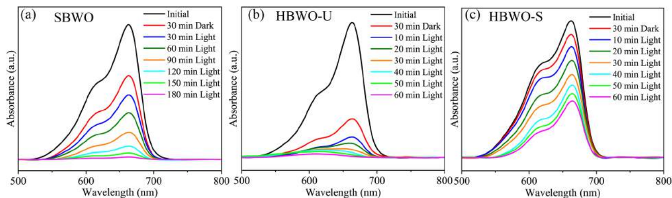
Fig. 8 The photocatalytic degradation measurements from UV-vis absorption spectra of (a) SBWO, (b) HBWO-U, and (c) HBWO-S photocatalysts ( 1 \text{ g L}^{-1} ) with 10 ppm MB dye.
