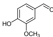
vanillin
