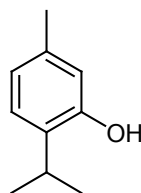
thymol
