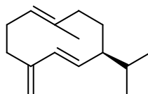
germacrene D
