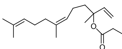
nerolidyl propionate
