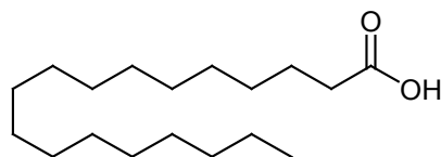
stearic acid
