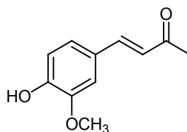
(E)-4-(4-hydroxy-3-methoxyphenyl)but-3-en-2-one
