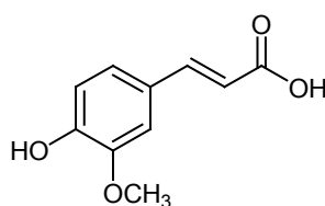
(E)-ferulic acid
