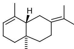
naphthalene, 1,2,3,4,4a,5,6,8a-octahydro-4a,8-dimethyl-2-(1-methylethylidene)
