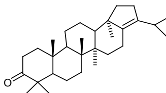
hopenone I
