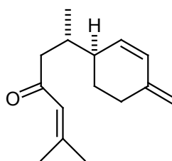
curlone
