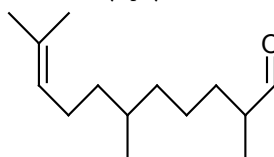
adoxal
