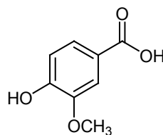
vanillic acid
