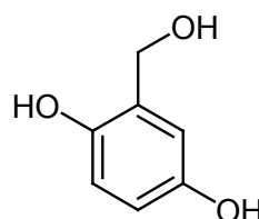
Structure of Gentisyl alcohol
