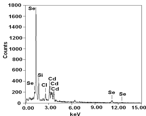
Fig. 3. EDX pattern of CdSe films on FTO surface.
