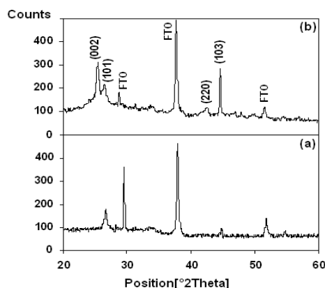
Fig. 4. X-ray diffraction pattern of (a) FTO surface and (b) as-deposited CdSe film.
