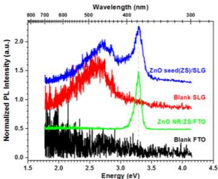
Figure 5. Normalized PL spectra (vertically offset for clarity) of ZS , ZnO NRs films, blank SLG, and blank FTO substrate recorded at room temperature. The PL intensity is normalized with respect to the highest peak height for all samples. The broad peak at ~2.6 eV (~490 nm) in panel originates from underlying SLG substrate.
