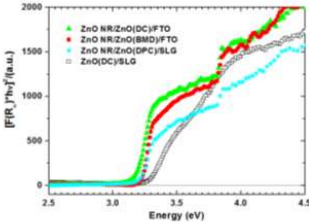
Figure 4. Tauc plot for estimating band gap using diffuse reflection data of ZnO(DC)/SLG (open rectangle), ZnO NR/ZnO(DPC)/SLG (solid star), ZnO NR/ZnO(BMD)/FTO (solid circle) and ZnO NR/ZnO(DC)/FTO (solid triangle) thin films.
